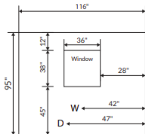
Example 2, Elevation
